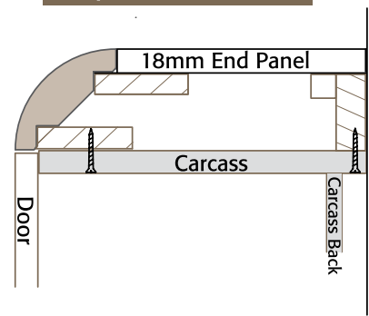
Step 2 - Fix to Carcass
