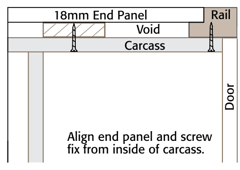
Step 2 - Fix to Carcass
