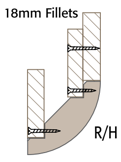
Step 1 - Fix 18mm Fillets to Rail
