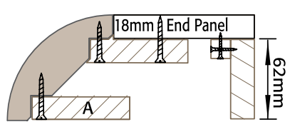
Step 1 - Assemble End Panel & Rail
