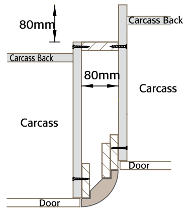
Step 2 - Fit to Carcass
